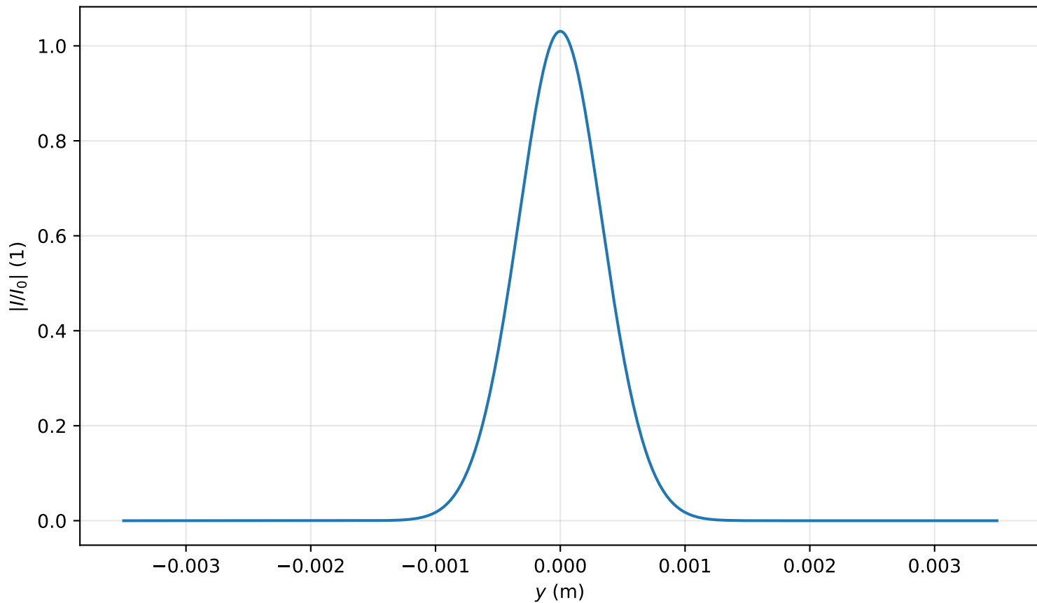
Intensity profile I(x=0, y, z=0.239)/I_0 , P_{in}=0.8P_{cr} , artificial time
